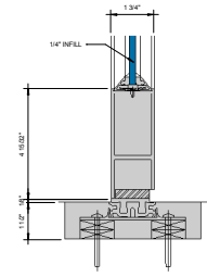
SECTION "B-B" 6" = 1'-0"
