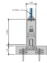
SECTION "C-C" 6" = 1'-0"
