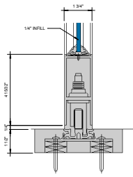
SECTION "A-A" 6" = 1'-0"
