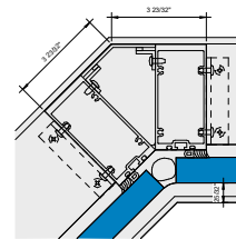
② Callout - Corner Inside 135 6\" = 1'-0"
