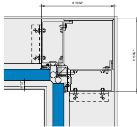
① Callout - Corner Inside 90 6\" = 1'-0"
