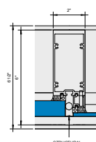
9 Callout - Outside Glazed Vertical 1 x 0.25" 6" = 1'-0"
