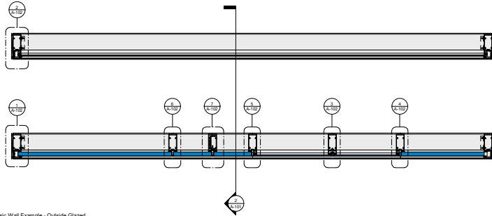
① Basic Wall Example - Outside Glazed 1 1/2" x 1'-0"
