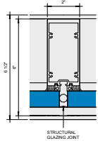
2 Callout - Outside Glazed Vertical 1 x 1" 6" = 1'-0"
