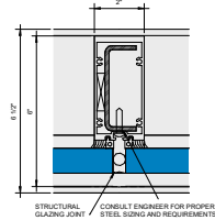
3 Callout - Outside Glazed Vertical Reinforced 1 x 1" 6" = 1'-0"
