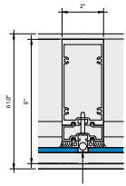
7 Callout - Outside Glazed Vertical 0.25 x 0.25" 6" = 1'-0"
