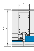
8 Callout - Outside Glazed Vertical 0.25 x 1" 6" = 1'-0"
