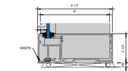
13 Callout - Sill 1/4" 6" = 1'-0"
