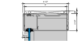
5 Callout - Outside Glazed Head 1/4" 6" = 1'-0"
