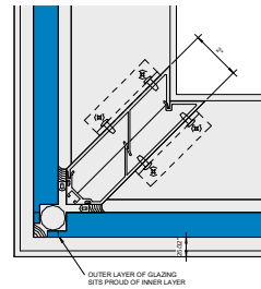
③ Callout - Corner 90 Dart 6\" = 1'-0"
