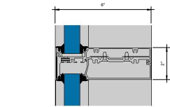
10 Callout - Horizontal 1 x 1" 6" = 1'-0"
