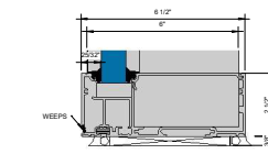
12 Callout - Sill 1" 6" = 1'-0"
