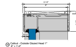
4 Callout - Outside Glazed Head 1/4" 6" = 1'-0"
