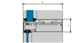
11 Callout - Horizontal 1 x 0.25" 6" = 1'-0"
