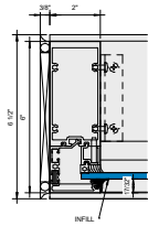
6 Callout - Outside Glazed Jamb 1/4" 6" = 1'-0"
