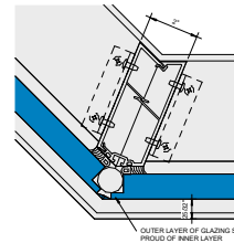
④ Callout - Corner 135 Dart 6\" = 1'-0"
