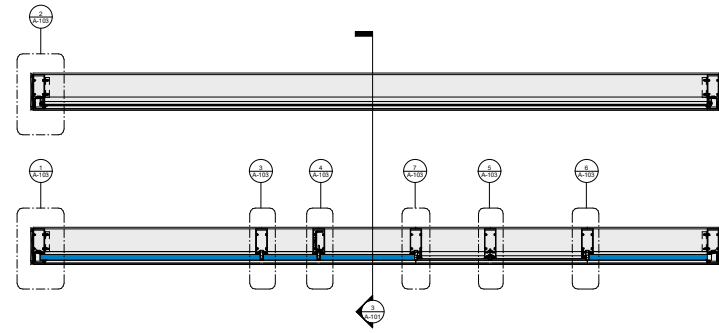
② Basic Wall Example - Inside Glazed 1 1/2" x 1'-0"
