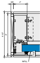
1 Callout - Outside Glazed Jamb 1" 6" = 1'-0"
