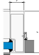
③ Callout - Door - Non-Thermal Jamb with Pocket Left 6' = 1'-0"
