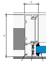
3 Callout - Window Vertical One Pocket Side 6" = 1'-0"
