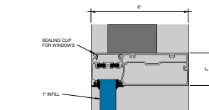
11 Callout - Window Inside Glazed - Intermediate Horizontal 111 6" = 1'-0"
