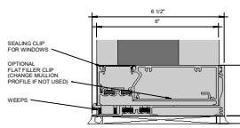
13 Callout - Window Outside Glazed Steps Up - Sill 103 6" = 1'-0"
