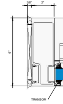
⑤ Callout - Door - Non-Thermal Transom Jamb 6' = 1'-0"
