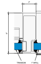
⑥ Callout - Door - Non-Thermal Transom Jamb with Pocket 6' = 1'-0"
