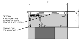
6 Callout - Window Outside Glazed - Head 003 6" = 1'-0"
