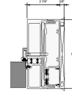
5 Callout - Door - Thermal Two Piece Jamb B 6" = 1'-0"
