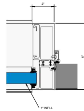
1 Callout - Door - Thermal Door Jamb with Pocket B 6" = 1'-0"
