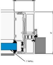
4 Callout - Door - Thermal Two Piece Door Jamb with Pocket B 6" = 1'-0"
