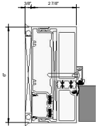
2 Callout - Door - Thermal Two Piece Jamb A 6" = 1'-0"
