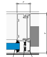
4 Callout - Window Vertical One Pocket Side 6" = 1'-0"
