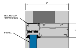
10 Callout - Window Outside Glazed Steps Up - Intermediate Horizontal 011A 6" = 1'-0"
