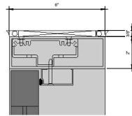
⑦ Callout - Door - Non-Thermal Head - CoC 6' = 1'-0"
