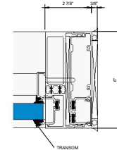
13 Callout - Door - Thermal Two Piece Transom Jamb B 6" = 1'-0"
