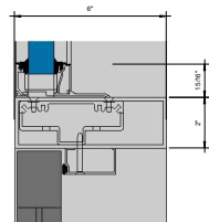
⑨ Callout - Door - Non-Thermal Transom Head - CoC 6' = 1'-0"
