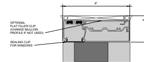
8 Callout - Window Inside Glazed - Head 003A 6" = 1'-0"
