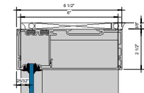
9 Callout - Outside Glazed Head 1/4" 6" = 1'-0"
