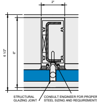
3 Callout - Outside Glazed Vertical Reinforced 1 x 1" 6" = 1'-0"
