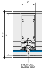
5 Callout - Outside Glazed Vertical 0.25 x 1.25" 6" = 1'-0"
