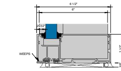
12 Callout - Sill 1" 6" = 1'-0"
