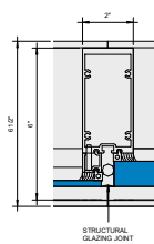
6 Callout - Outside Glazed Vertical 0.25 x 1" 6" = 1'-0"
