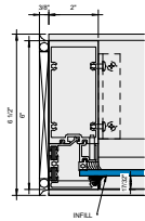
4 Callout - Outside Glazed Jamb 1/4" 6" = 1'-0"
