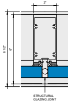
2 Callout - Outside Glazed Vertical 1 x 1" 6" = 1'-0"
