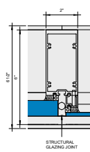
7 Callout - Outside Glazed Vertical 1 x 0.25" 6" = 1'-0"
