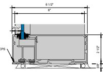
13 Callout - Sill 1/4" 6" = 1'-0"
