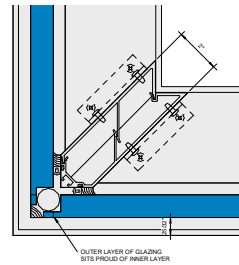
2 Callout - Corner 90 Dart 6" = 1'-0"
