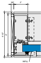
1 Callout - Outside Glazed Jamb 1\"/>
