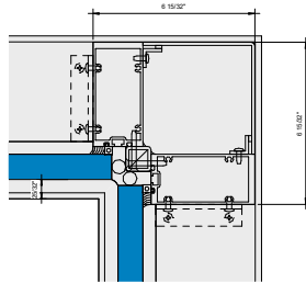
1 Callout - Corner Inside 90 6" = 1'-0"
