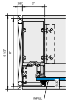
4 Callout - Outside Glazed Jamb 1/4\"/>
