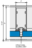
2 Callout - Outside Glazed Vertical 1 x 1\"/>
