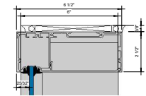
9 Callout - Outside Glazed Head 1/4\"/>
