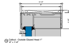
8 Callout - Outside Glazed Head 1\"/>
