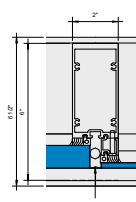
7 Callout - Outside Glazed Vertical 1 x 0.25\"/>
