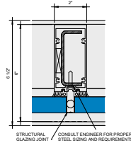
3 Callout - Outside Glazed Vertical Reinforced 1 x 1\"/>
