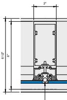
5 Callout - Outside Glazed Vertical 0.25 x 0.25\"/>
