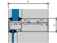
11 Callout - Horizontal 1 x 0.25\"/>
