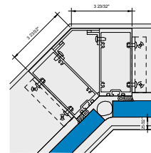
3 Callout - Corner Inside 135 6" = 1'-0"
