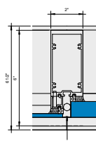
6 Callout - Outside Glazed Vertical 0.25 x 1\"/>
