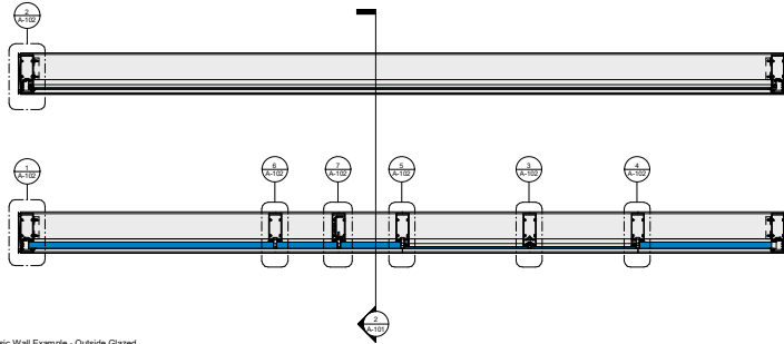
1 Basic Wall Example - Outside Glazed 1 1/2" x 1-0"
