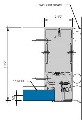
⑤ SSG JAMB - 1" INFILL 6" = 1'-0"
