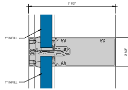
② HORIZONTAL - 1" INFILL 6" = 1'-0"
