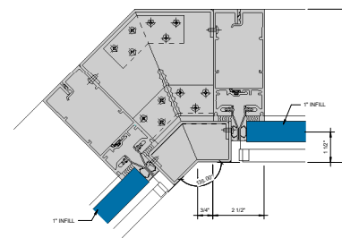
⑩ 135° INSIDE CORNER - 1" INFILL 6" = 1'-0"
