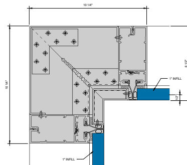
⑨ SSG 90° INSIDE CORNER - 1" INFILL 6" = 1'-0"
