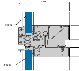
③ EXPANSION HORIZONTAL - 1" INFILL 6" = 1'-0"
