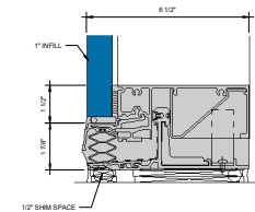
④ SSG SILL - 1" INFILL 6" = 1'-0"
