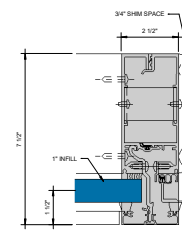
③ EXPANSION HORIZONTAL - 1" INFILL 6" = 1'-0"
