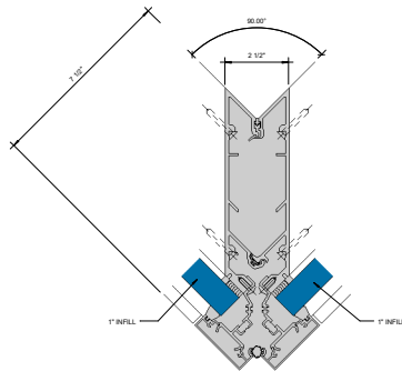
⑧ 90° OUTSIDE CORNER - 1" INFILL 6" = 1'-0"
