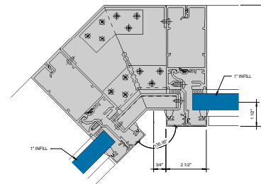
⑩ 135° OUTSIDE CORNER - 1" INFILL 6" = 1'-0"
