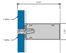
② SSG HORIZONTAL - 1" INFILL 6" = 1'-0"
