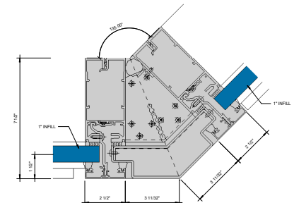
⑪ 135° INSIDE CORNER - 1" INFILL 6" = 1'-0"
