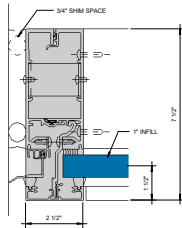
① HEAD - 1" INFILL 6" = 1'-0"
