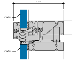
③ EXPANSION HORIZONTAL - 1" INFILL 6" = 1'-0"
