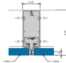
⑥ SSG VERTICAL MULLION - 1" INFILL 6" = 1'-0"
