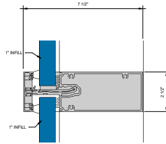
② HORIZONTAL - 1" INFILL 6" = 1'-0"
