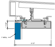
① SSG HEAD - 1" INFILL 6" = 1'-0"
