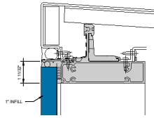
① SSG HEAD - 1" INFILL 6" = 1'-0"
