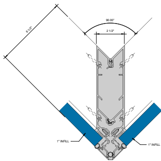
⑧ SSG 90° OUTSIDE CORNER - 1" INFILL 6" = 1'-0"
