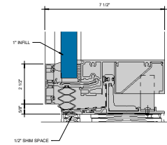
④ SILL - 1" INFILL 6" = 1'-0"
