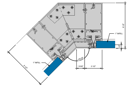
⑪ SSG 135° INSIDE CORNER - 1" INFILL 6" = 1'-0"
