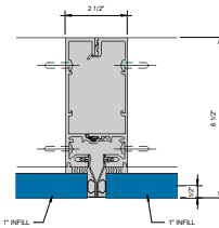
⑥ SSG VERTICAL MULLION - 1" INFILL 6" = 1'-0"
