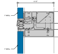
③ SSG EXPANSION HORIZONTAL - 1" INFILL 6" = 1'-0"
