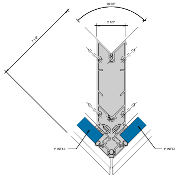
⑧ 90° OUTSIDE CORNER - 1" INFILL 6" = 1'-0"
