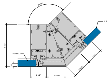
⑩ SSG 135° OUTSIDE CORNER - 1" INFILL 6" = 1'-0"
