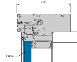
③ HEAD COS - 1\"/>
