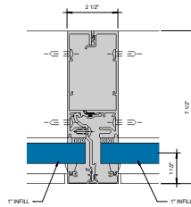
⑥ VERTICAL MULLION - 1" INFILL 6" = 1'-0"
