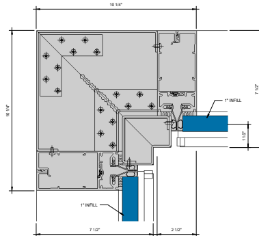
⑨ 90° INSIDE CORNER - 1" INFILL 6" = 1'-0"
