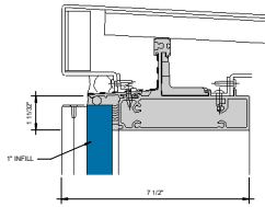
① HEAD - 1" INFILL 6" = 1'-0"
