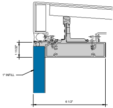
① SGT HEAD - 1" INFILL 6" x 1'-0"
