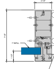
⑦ JAMB - 1" INFILL 6" = 1'-0"
