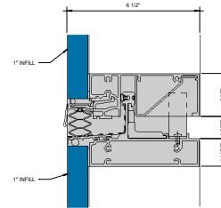
③ SGT EXPANSION HORIZONTAL - 1" INFILL 6" x 1'-0"
