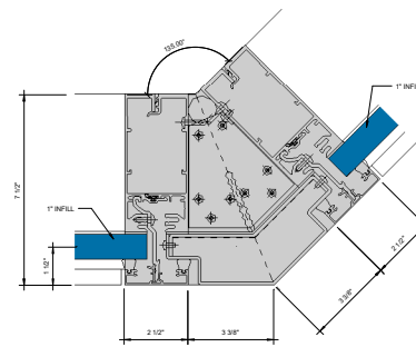
⑩ 135° OUTSIDE CORNER - 1" INFILL 6" = 1'-0"
