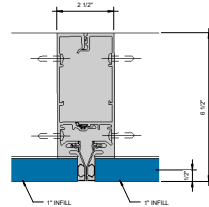
⑥ SGT VERTICAL MULLION - 1" INFILL 6" x 1'-0"
