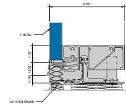
④ SGT SILL - 1" INFILL 6" x 1'-0"
