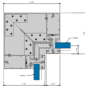
⑨ 90° INSIDE CORNER - 1" INFILL 6" = 1'-0"
