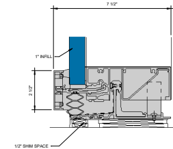
④ SILL - 1" INFILL 6" = 1'-0"
