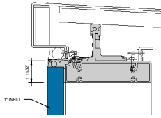
① HEAD - 1" INFILL 6" = 1'-0"
