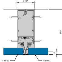
⑥ SGT VERTICAL MULLION - 1" INFILL 6" = 1'-0"
