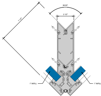
⑧ 90° OUTSIDE CORNER - 1" INFILL 6" = 1'-0"
