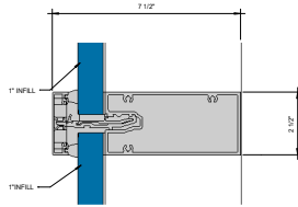
② HORIZONTAL - 1" INFILL 6" = 1'-0"
