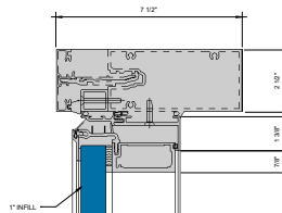
⑦ HEAD-PO-1" INFILL S = 1'-0"
