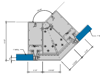
⑩ SGT 135° OUTSIDE CORNER - 1" INFILL 6" x 1'-0"
