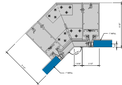
⑪ SGT 135° INSIDE CORNER - 1" INFILL 6" x 1'-0"
