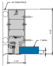
⑤ SGT JAMB - 1" INFILL 6" = 1'-0"
