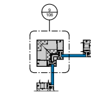
90° INSIDE CORNER - 1" INFILL 1" = 1'-0"
