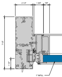
④ LEFT JAMB-COS-1" INFILL S = 1'-0"
