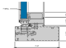
⑤ SILL - 1" INFILL S = 1'-0"
