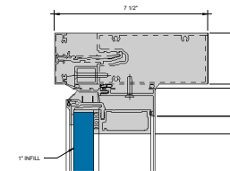
⑥ HEAD-COS-1" INFILL S = 1'-0"
