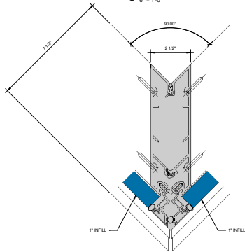
⑤ SGT JAMB - 1" INFILL 6" = 1'-0"
