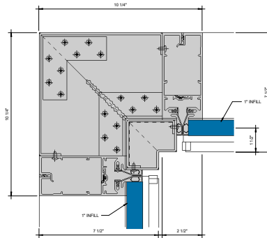
⑨ 90° INSIDE CORNER - 1" INFILL 6" = 1'-0"
