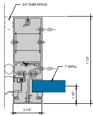
⑤ JAMB - 1" INFILL 6" = 1'-0"
