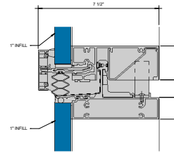
③ EXPANSION HORIZONTAL - 1" INFILL 6" = 1'-0"
