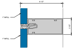
② SGT HORIZONTAL - 1" INFILL 6" x 1'-0"
