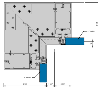
⑨ SGT 90° INSIDE CORNER - 1" INFILL 6" x 1'-0"
