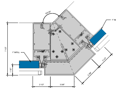
⑩ 135° OUTSIDE CORNER - 1" INFILL 6" = 1'-0"
