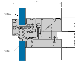
③ EXPANSION HORIZONTAL - 1" INFILL 6" = 1'-0"
