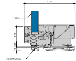
④ SILL - 1" INFILL 6" = 1'-0"
