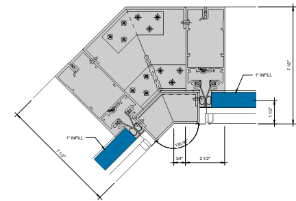
⑪ 135° INSIDE CORNER - 1" INFILL 6" = 1'-0"
