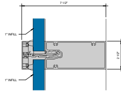
② HORIZONTAL - 1" INFILL 6" = 1'-0"
