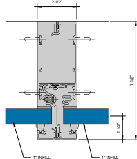
⑥ VERTICAL MULLION - 1" INFILL 6" = 1'-0"
